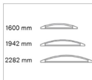
ROOF PANELS Bus shelter roof width options: 1600mm 1942mm 2282mmw
