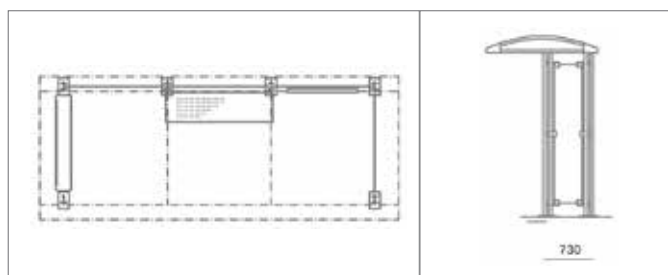
97101503 Bus shelter with 3 modules with CITY LIGHT, timetable plan and bench
