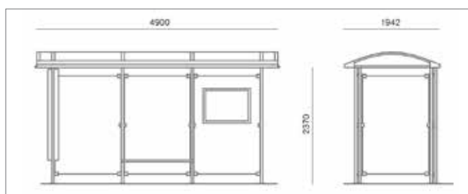
97101608 Bus shelter 101 608 304 Stainless steel frame 8 modules 10mm safety glass panels
