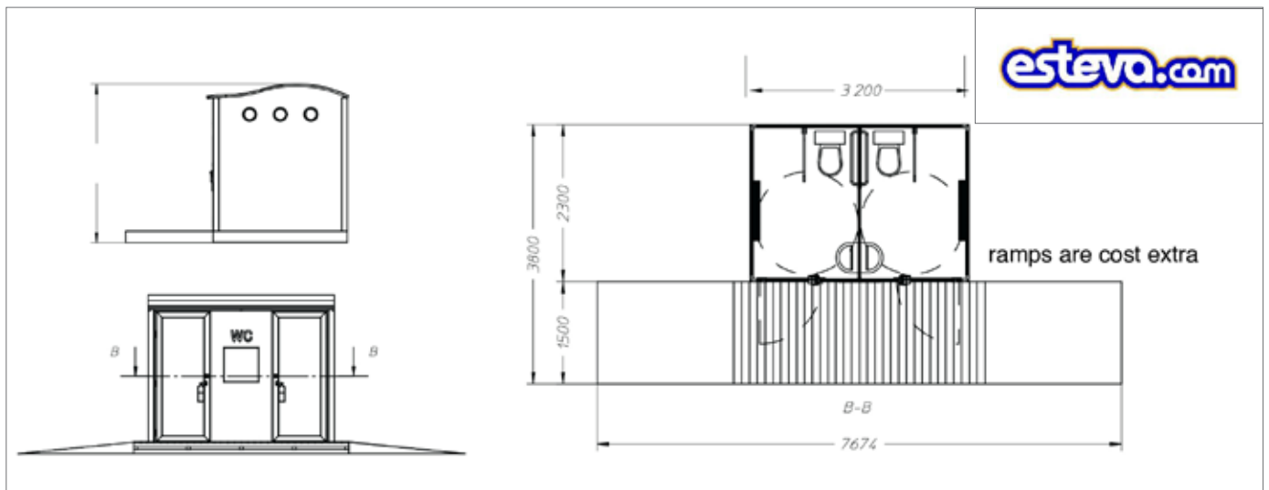
51580 - 3200x2300x2175h overseas model shown
